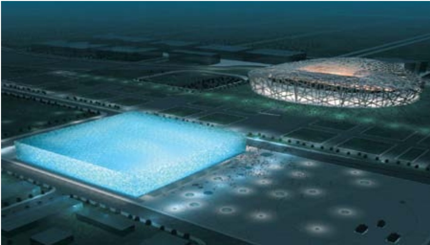
Figure 5: PTW Architects, CSCEG Design and Arup, 'Watercube' National Swimming Centre, Beijing, due for completion 2007 Competition model showing overall scale: 177 x 177 metres (581 x 581 feet) and more than 30 metres (98 feet) high, with an entirely column-free interior space.
