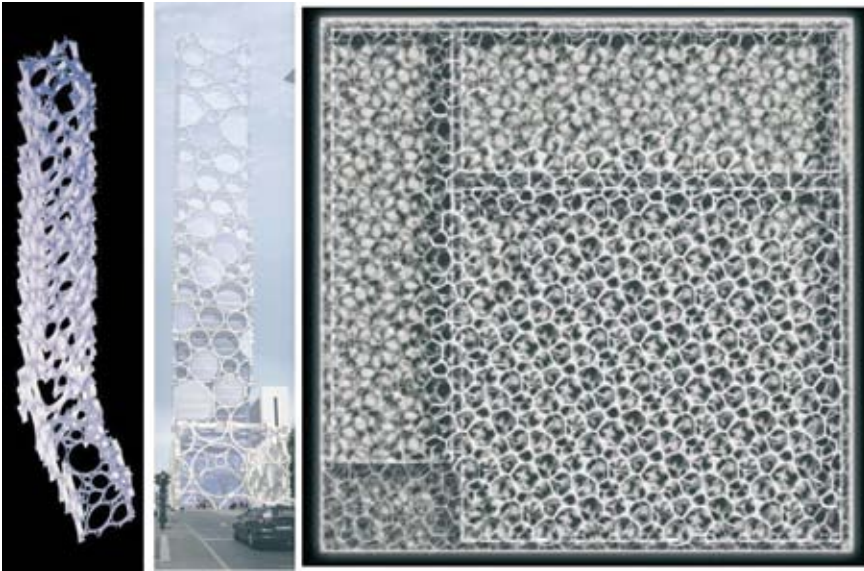
Figure 4: (left) SMO Architektur and Arup, Bubble Highrise, Berlin, 2002, (Right) Watercube digital structural model. The mathematics of foam geometries are used to produce the structural array, ensuring a rational optimised and buildable structural geometry.
